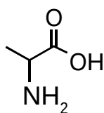
Alanina
