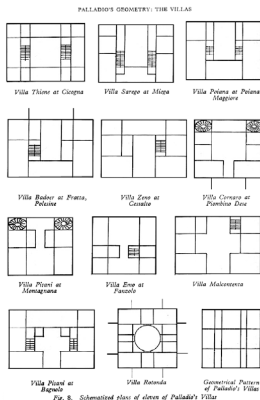
Fig. 8. Schematized plans of eleven of Palladio's Villas
