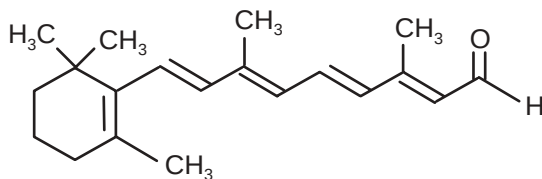
Retinal
