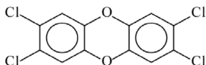
2,3,7,8-tetraclorodibenzo-p-dioxina (2,3,7,8-TCDD)
