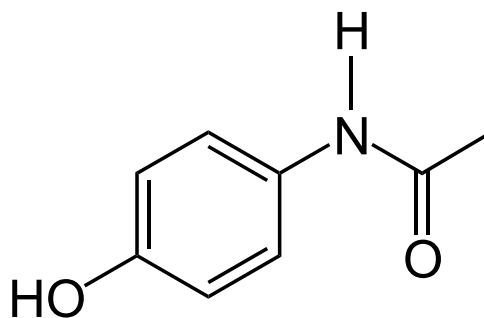
Paracetamol
