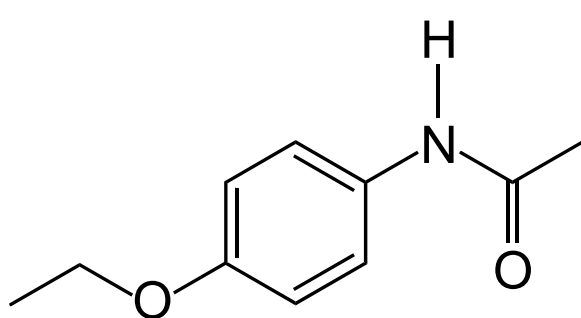
Fenacetina
