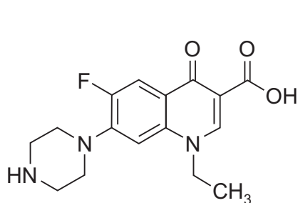
norfloxacin
