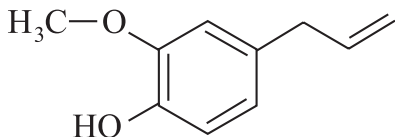
Eugenol
