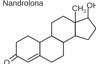
Nandrolona
