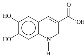
melanina
