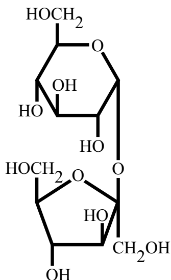
Sacarose
