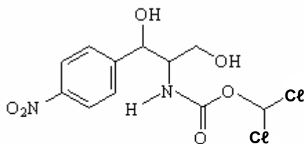
Cloranfenicol
