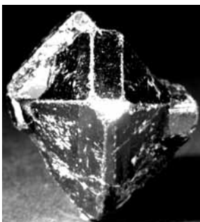
cassiterita ( \text{SnO}_2 )
